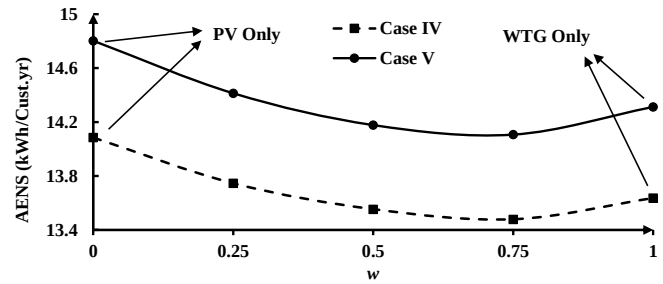
Fig. 8. AENS vs. the mix of RESs in Cases IV-V.
