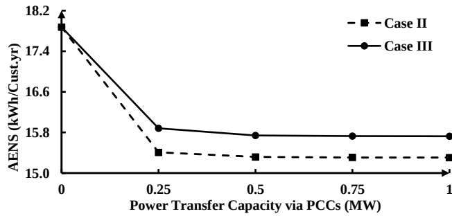
Fig. 6. AENS vs. power transfer capacity in Cases II-III.
