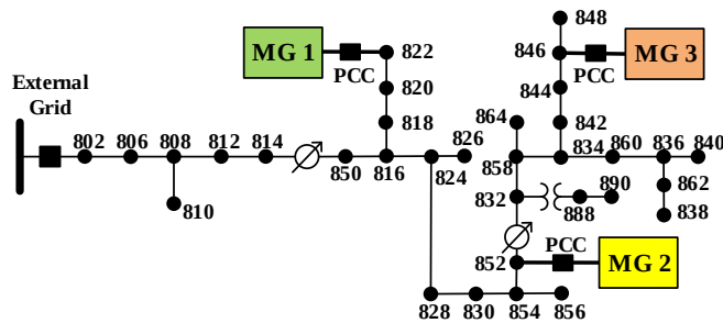
Fig. 5. Single line diagram of the system under study.
