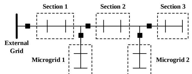
Fig. 1. Sample system for illustrating different operating modes.
