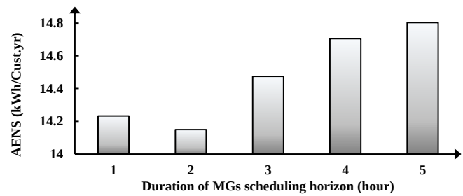
Fig. 9. AENS vs. duration of scheduling horizon in Case V.
