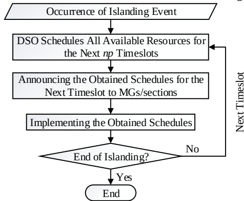
Fig. 3. The proposed centralized outage management scheme.
