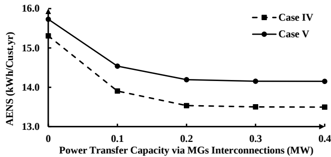
Fig. 7. AENS vs. power transfer capacity in Cases IV-V.
