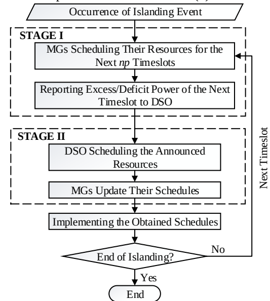
Fig. 4. The presented decentralized outage management scheme.
